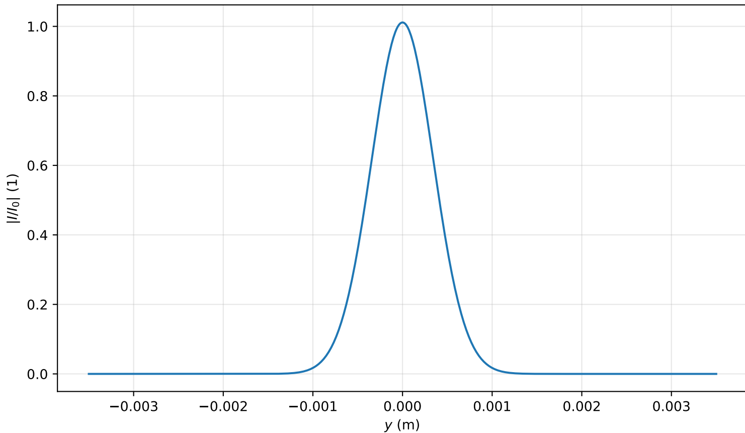
Intensity profile I(x=0, y, z=0.159)/I_0 , P_{in}=0.7P_{cr} , artificial time
